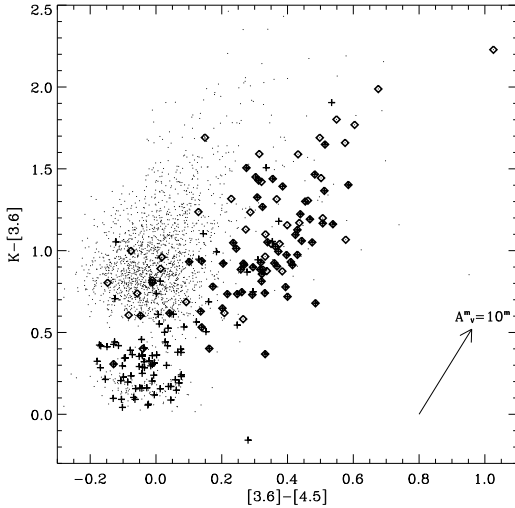
Fig. 12. Color-color diagram with K and IRAC bands for the stars in ACIS FOV (points). Diamonds are stars with excesses in 2MASS bands detected with Q_{2\text{MASS}} indices defined in GPM07, while crosses mark X-ray sources. The reddening vector, corresponding to A_V = 10^m , has been obtained from the extinction law of Megeath et al. (2004).
