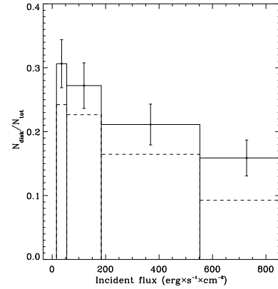
Fig. 13. Percentage of members with disks in the ACIS FOV vs. the estimated incident flux from OB members. The four values are 31\% \pm 4\% , 27\% \pm 4\% , 21\% \pm 3\% , and finally 16\% \pm 3\% , from left to the right.
