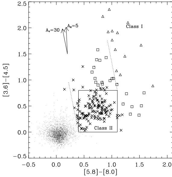
Fig. 3. Color-color diagram for IRAC sources in WFI FOV (dots). The box marks the approximate locus of Class II YSOs (crosses). The dashed lines roughly separate reddened photospheres (left), reddened Class II YSOs (center), and Class I YSOs (in the upper right part of the diagram, marked with triangles). Squares mark stars either classifiable as Class II or Class I YSOs. The reddening vectors with A_V = 30^m and A_K = 5^m are obtained from Megeath et al. (2004) and Flaherty et al. (2007), respectively.
