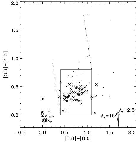
Fig. 5. IRAC color-color diagram of the X-ray sources (crosses). Dots mark the stars with disks selected from the IRAC diagram of Fig. 3, for the sky region contained in the ACIS FOV. The Class II locus and the reddening vectors are analogous to those in Fig. 3.
