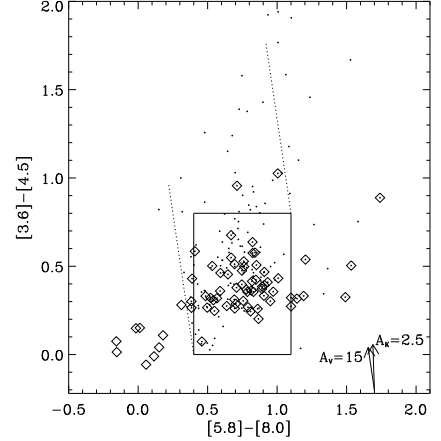
Fig. 10. IRAC color-color diagrams of the stars with disks selected with the IRAC diagram of Fig. 3 (points) and of the stars with excesses in 2MASS bands selected in GPM07 (diamonds). The Class II locus and the reddening vectors are analogous to those in Fig. 3.
