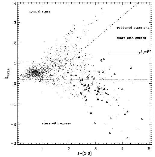
Fig. 11. Diagram Q_{VIJ[3.6]} vs. J-[3.6] for the stars in the WFI FOV, with overplotted the stars with excesses selected with the IRAC color-color diagram (triangles).
