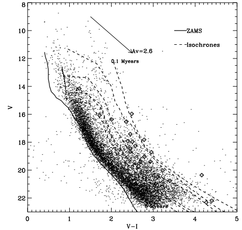
Fig. 4. V vs. V - I diagram analogous to that in Fig. 2. Diamonds mark candidate stars with disks selected by the IRAC color-color diagram but not in GPM07.
