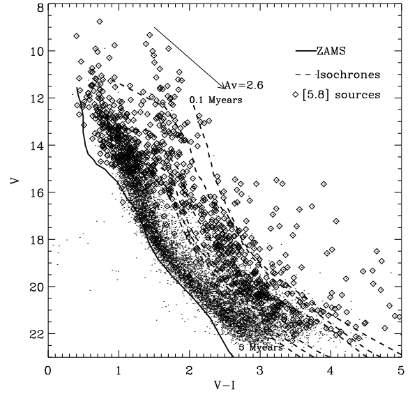
Fig. 2. V vs. V - I diagram of stars in WFI FOV. The thick solid line is the ZAMS (from Siess et al. 2000), at the distance of 1750 pc and with A_V = 1.45^m (the average extinction of field stars, evaluated in GPM07). The dashed lines are the isochrones at 0.1, 0.25, 1, 2.5, 3, and 5 Myr, with the average extinction appropriate for cluster members ( A_V = 2.6^m ). The extinction vector is obtained from the law of Munari & Carraro (1996). The diamonds are optical sources detected at 5.8 \mu\text{m} .
