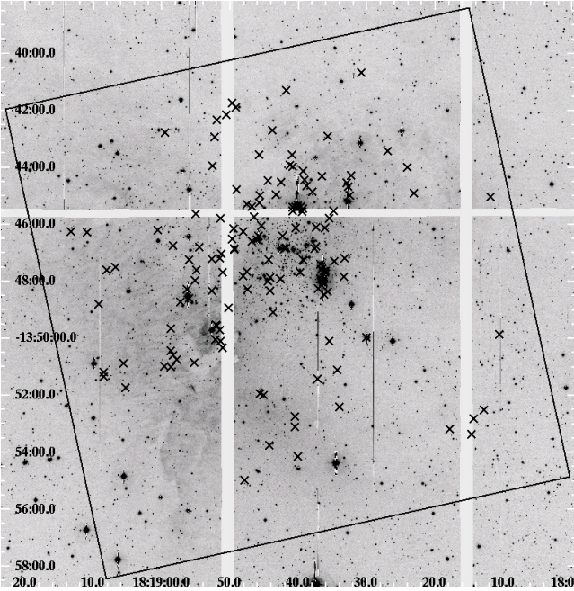
Fig. 1. WFI image, in the I band, of the central region of NGC 6611. Crosses identify the X-ray sources without both optical and infrared counterpart. The box outlines the 17' \times 17' ACIS FOV.
