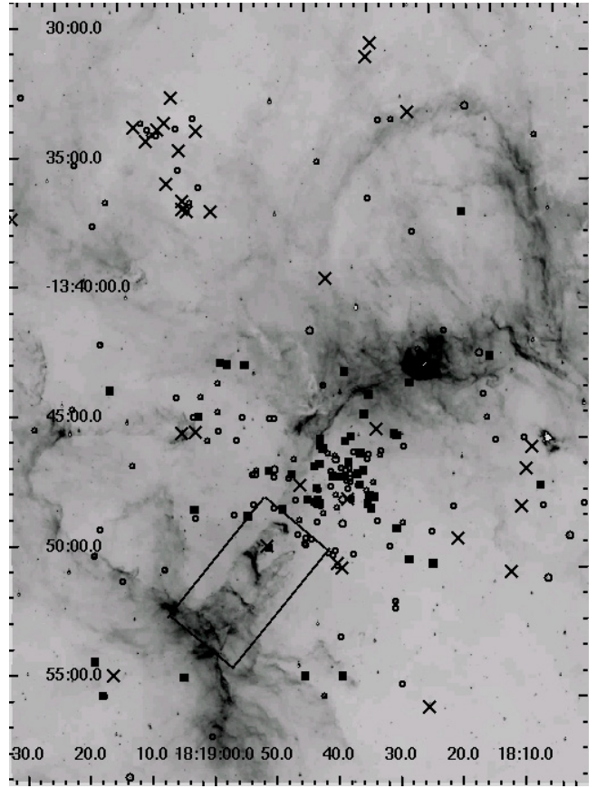
Fig. 6. IRAC image of the Eagle Nebula at 8.0 \mu m , centered on the cluster and covering approximately a region of 22' \times 32' . The circles mark Class II YSOs, while the crosses mark Class I YSOs and stars consistent with both classifications. The small boxes mark massive stars. The box delimits the structures known as “elephant trunks”. North is up, East is to the left.
