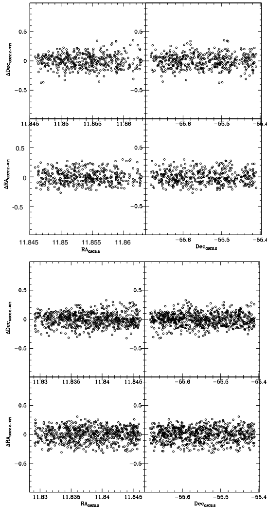
Fig. 3. Positional residuals, computed as in Fig. 2, as a function of RA and Dec in the GSC 2.2 reference catalogue. The results refer to chips 2 ( left panel ) and 3 ( right panel ), where the cluster is mainly concentrated.
