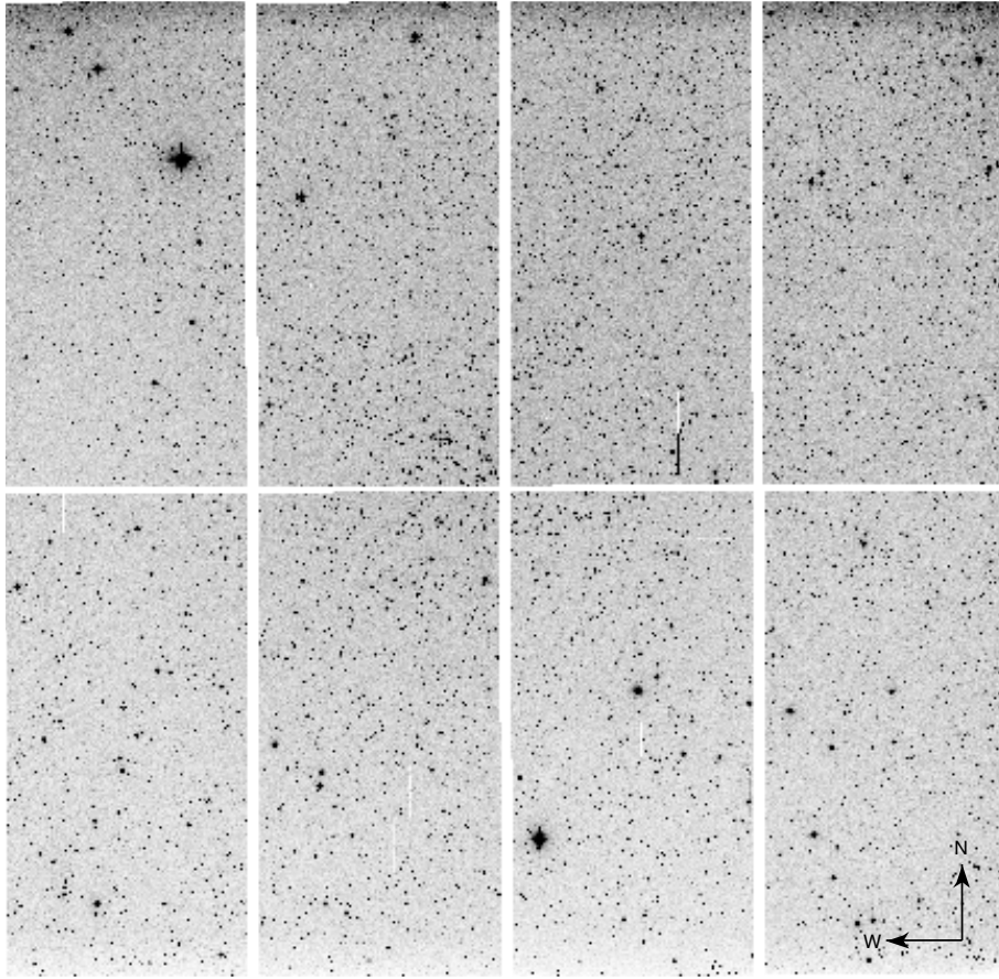
Fig. 1. A deep WFI image of the region around NGC 3960 taken in the B filter. The field center is RA = 11^h50^m51^s.6 and Dec = -55^\circ42'07'' (J2000). Each chip is 8'.12 \times 16'.25 , while the full field of view is 34' \times 33' . The cluster is located approximately in the central part of the field of view where it is barely visible; it has a radius of about 7 arcmin. Strong effects of differential reddening cause a non-uniform spatial distribution of the field stars in the external regions of the field of view.
