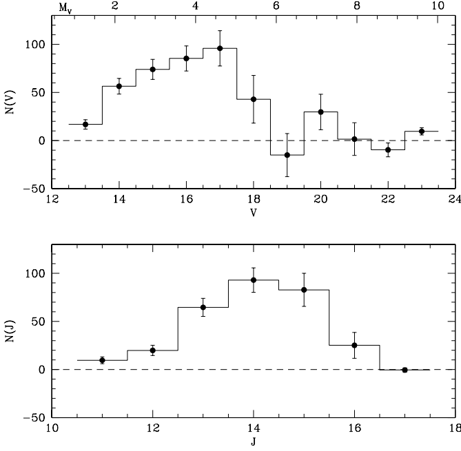
Fig. 15. Luminosity functions of NGC 3960, corrected for the field star contribution, obtained from optical data ( top panel ) and from IR data ( bottom panel ). The dashed lines indicate the zero values of the distributions.
