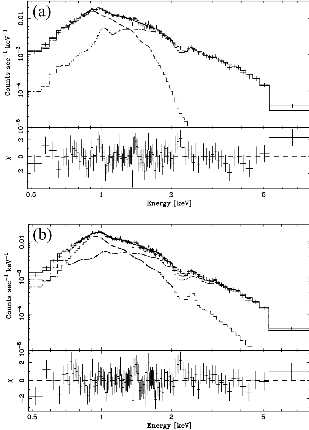
FIG. 6.—Spectrum of COUP source 567 exemplifying a common ambiguity in spectral fitting. Panel (a) presents a fit with kT_1 \approx 0.2 keV, kT_2 \approx 1.7 keV, \log N_H \approx 21.8 cm ^{-2} , and \log L_{t,c} \approx 31.6 ergs s ^{-1} with a reduced \chi^2 \approx 1.3 . Panel (b) presents another fit (which appears in Table 6) with kT_1 \approx 0.8 keV, kT_2 \approx 3.1 keV, \log N_H \approx 21.3 cm ^{-2} , \log L_{t,c} \approx 30.6 ergs s ^{-1} , and a reduced \chi^2 \approx 1.4 . Note the tenfold difference in inferred unabsorbed luminosity in the total 0.5–8 keV band.
